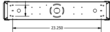
2' End Dimensions
