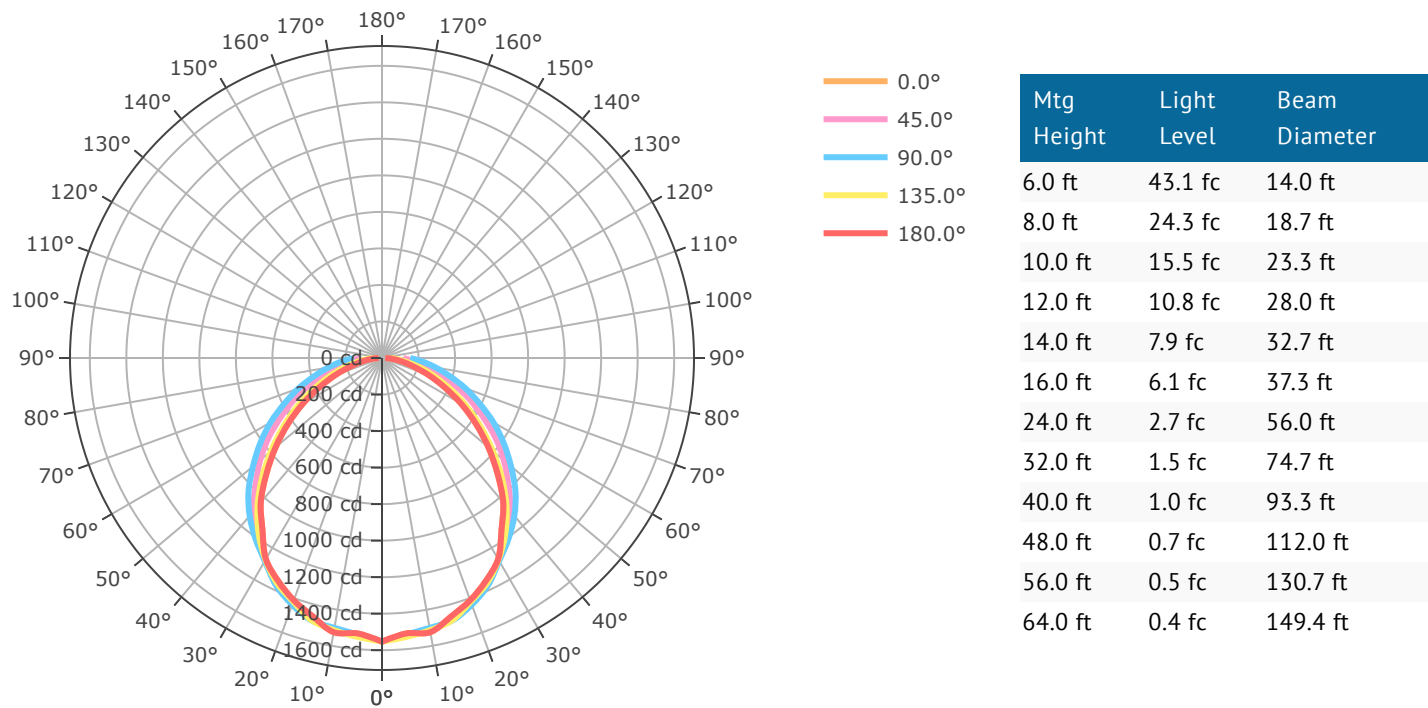
BRLS-4'-4L-840
