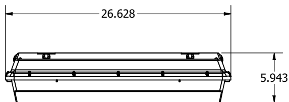
BLHV 2' Lateral
