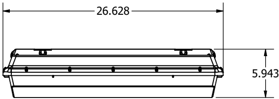
BLHV 2' Lateral
