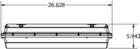
BLHV-H27 2' Lateral
