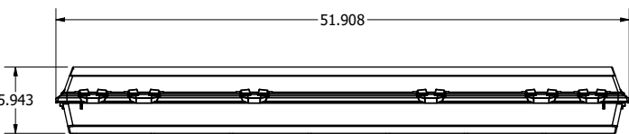
BLHV-H27 4' Lateral
